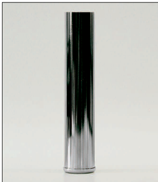
D 2 Metallfuss rund, hochglanz verchromt Ø 30 mm, 160 mm hoch Metal leg, round, highly polished chromium-plated Ø 30 mm, height 160 mm
